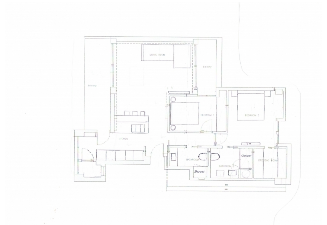
Floor plan
